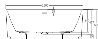
ROS 15075BTW 1500x750x585
