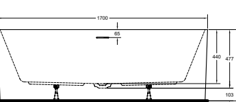
ALP 17075BTW 1700x745x580
