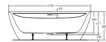
CAS 17080S 1700x800x585
