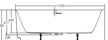
ROS 17080RH 1700x800x585
