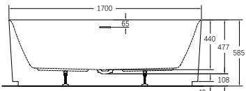
ROS 17080S 1700x800x585
