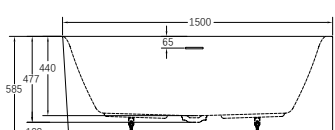
ROS 15075RH 1500x750x585
