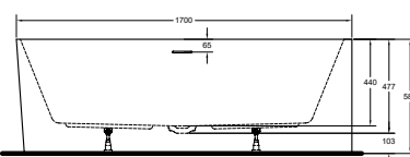
ALP 17075RH 1700x745x580
