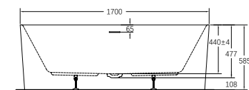
DEC 17075BTW 1700x750x585
