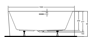
ALP 15075RH 1500x745x580
