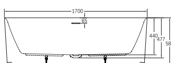
ROS 17080BTW 1700x800x585
