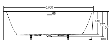
ROS 17080LH 1700x800x585
