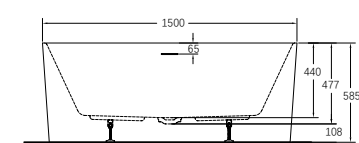
DEC 15075BTW 1500x750x585
