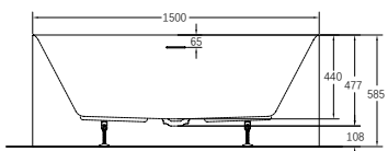
LUN 15073BTW 1500x730x585
