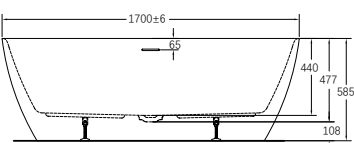
NEW 17080BTW 1700x800x585
