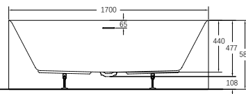
LUN 17075BTW 1700x750x585
