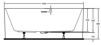
ALP 15075BTW 1500x745x580
